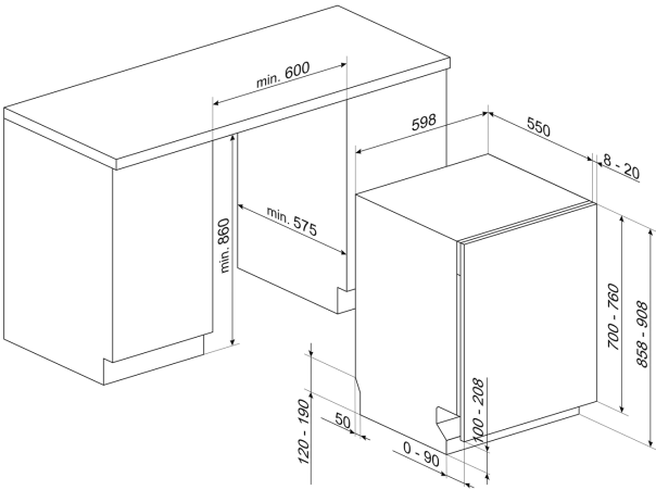
KITPL60N Black toe kick adjustable in height and depth for underbenck dishwashers
